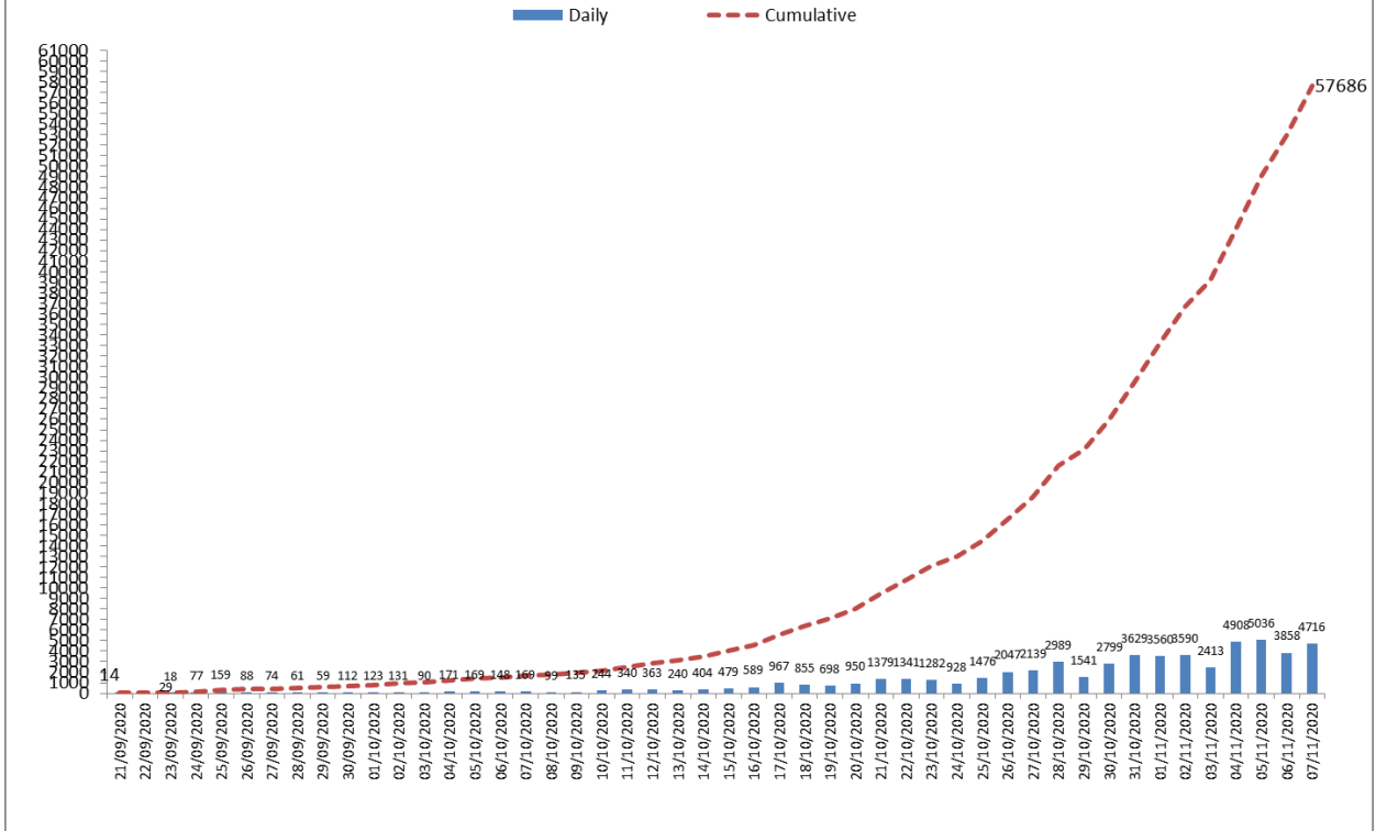
Temporal Distribution of Active Fire Events (Paddy) 2020 Period: 21 September to 07 November
